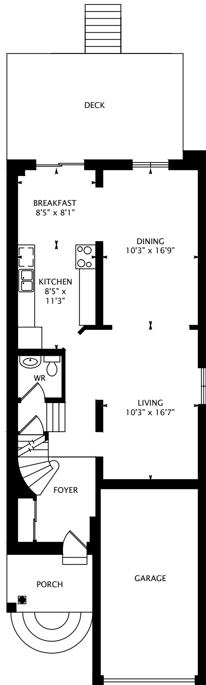
MAIN FLOOR 842 SQUARE FEET
